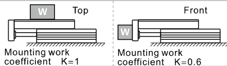
Fig 2: Mounting work coefficient (K)
